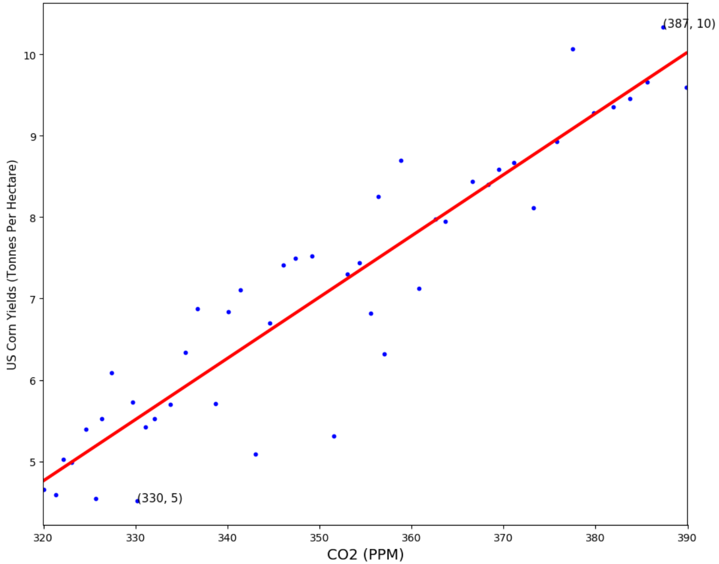
US Corn Yields (Tonnes Per Hectare) Vs. CO2
