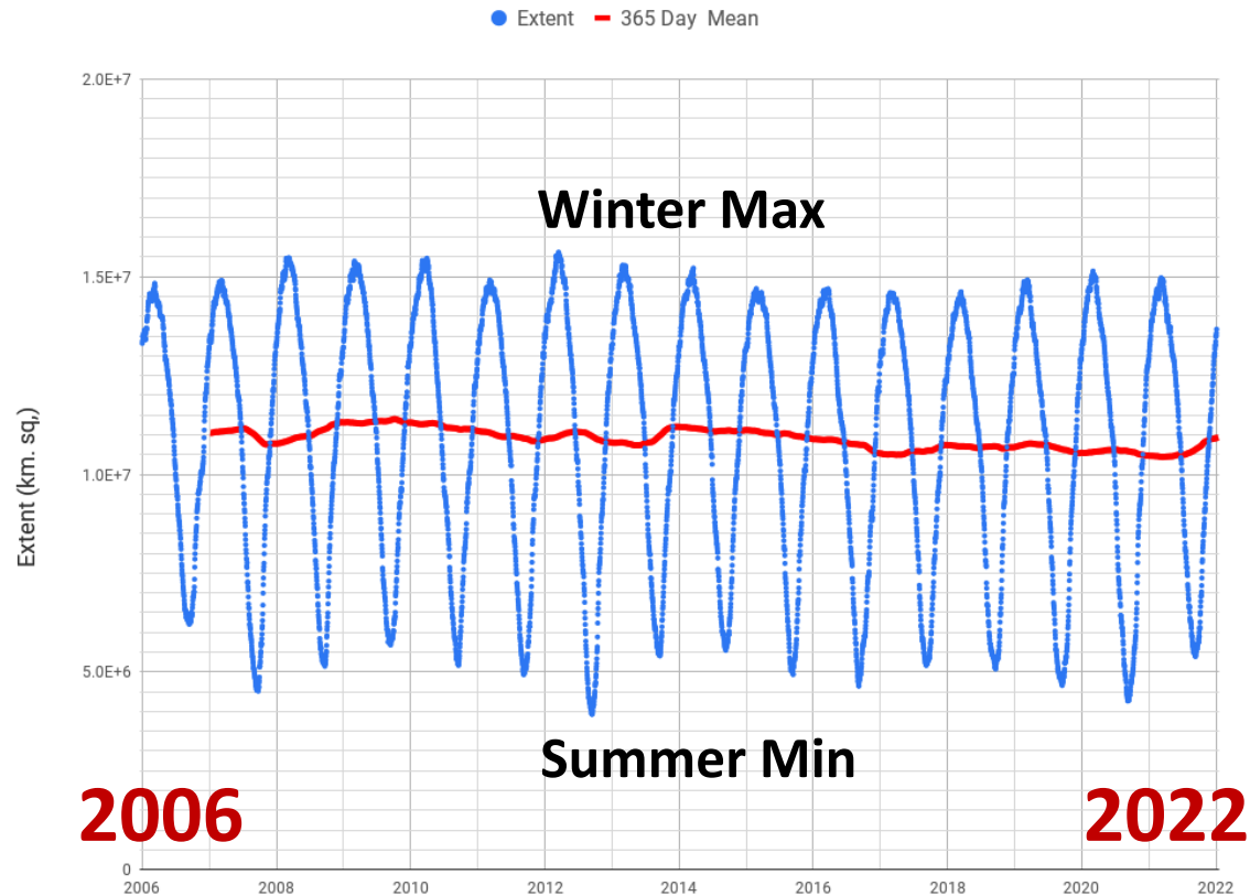
OSI Arctic Sea Ice Extent
